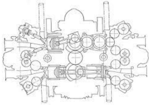
BRM 16 cylinder
