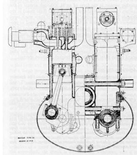
Twin Crankshaft U16 engine design
